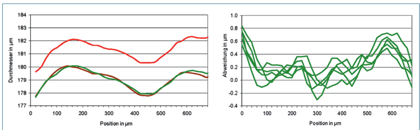
Figure 7. After correcting the CT measurement of the diameter (curve along the injection hole) of a diesel injection nozzle (left, red) by means of a reference measurement with the Werth Fiber Probe (left, brown) the measuring deviations of several corrected CT measurements (right) stay below one micron.
