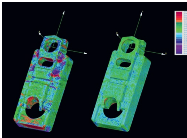
Figure 5. In comparison with the measurement without Virtual Artifact Correction, VAC (left), the measurement deviations with VAC (right) are significantly reduced.
