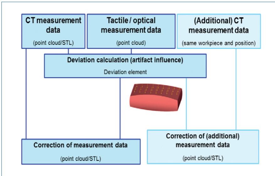
Figure 6. Principle of “Multisensor Autocorrection”
