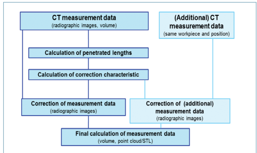
Figure 2. Principle of "Empirical Artifact Correction" (EAC)
