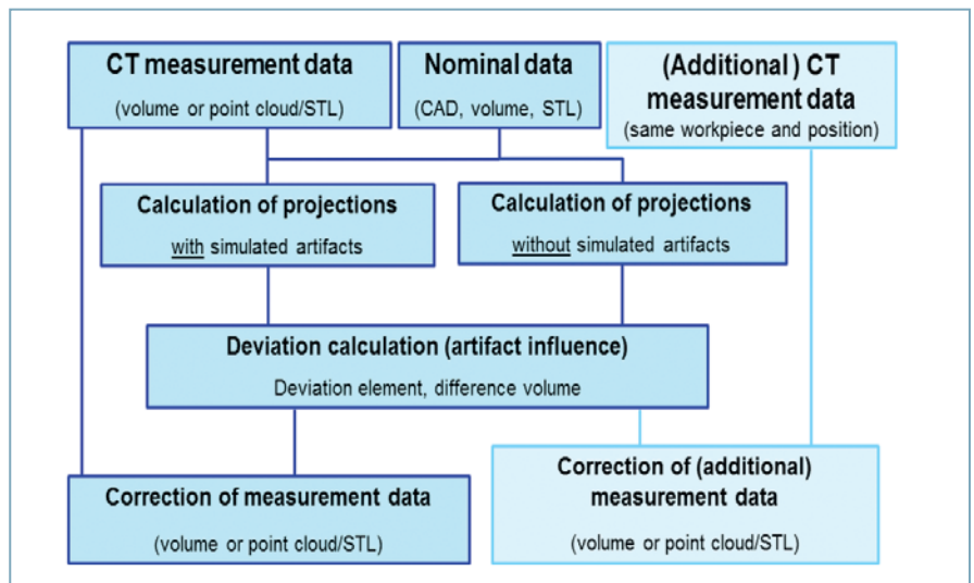
Figure 4. Principle of “Virtual Autocorrection” (VAC)
